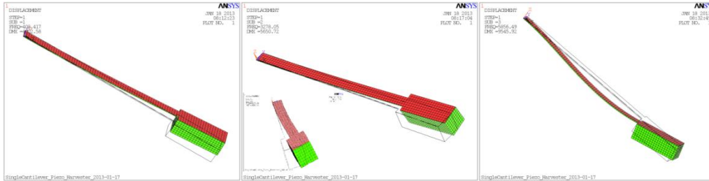
Figure 5. The First Three Modes
