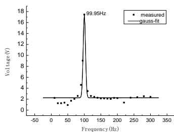
Figure 23. Frequency Response Curve (External Resistor 100KΩ)
