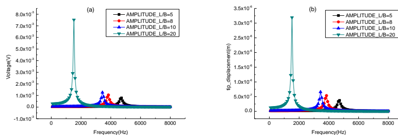
Figure 10. The Effect of Length to Width Ratio
