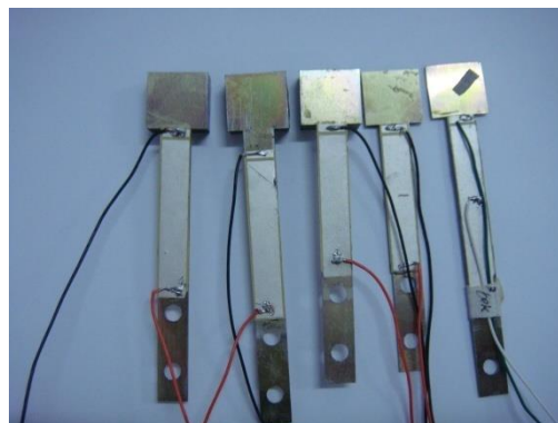
Figure 16. Harvester and Wiring
