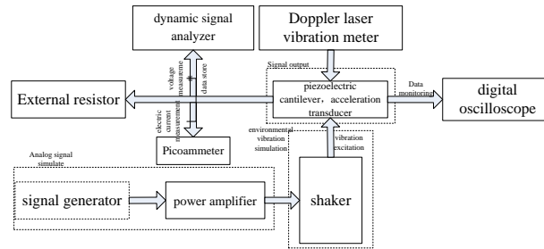
Figure 12. The Architecture of the Measurement
