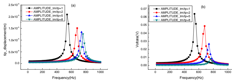
Figure 11. The Effect Substrate Thickness to Piezoelectric Thickness Ratio
