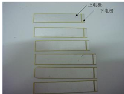
Figure 15. Piezoelectric Patch
