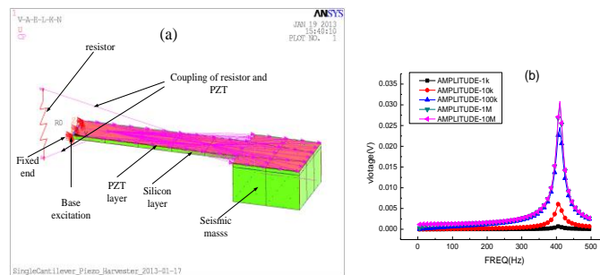
Figure 7. The Coupling Molding and the Voltage of Out Circuit When Connect Different Resistor
