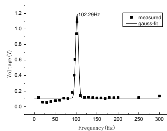
Figure 21. Frequency Response Curve (External Resistor 1KΩ)
