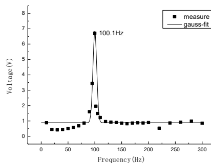
Figure 22. Frequency Response Curve (External Resistor 10KΩ)
