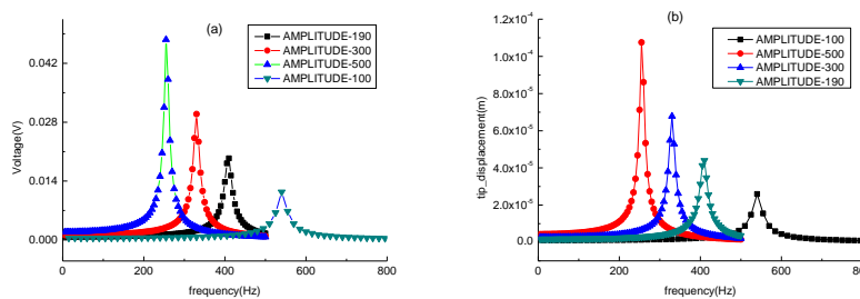
Figure 12. The Effect of Seismic Mass
