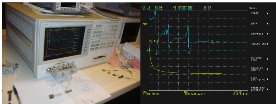
Figure 25. Resistance Measurement of Piezoelectric and the Result
