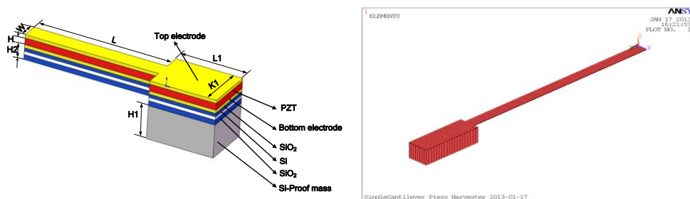
Figure 1. Diagram of Cantilever Structure
