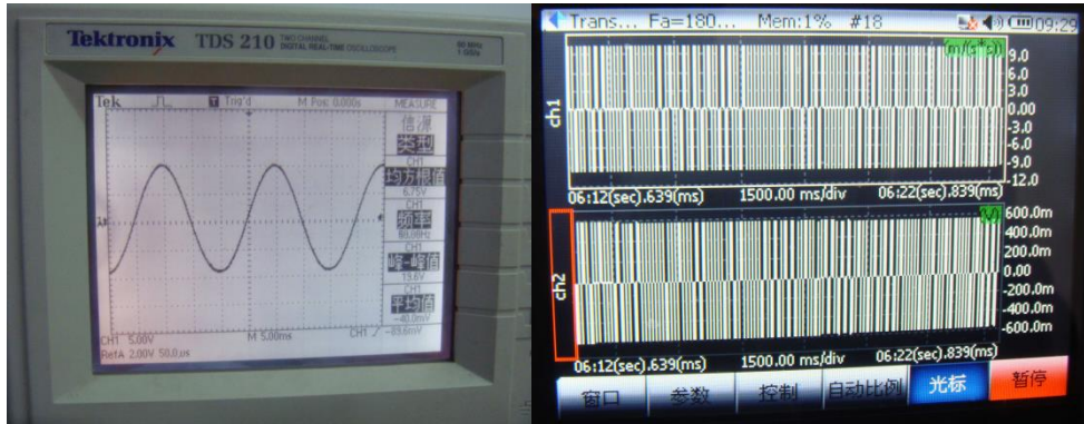
Figure 17. AC Voltage and the Acceleration and Voltage
