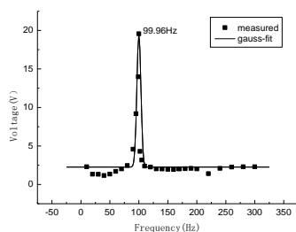
Figure 24. Frequency Response Curve (External Resistor 1MΩ)
