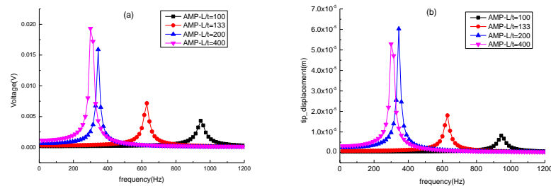
Figure 9. The Effect of Different Length to Thickness Ratio
