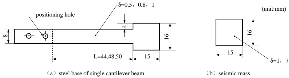
Figure 14. Geometry of the Single Cantilever
