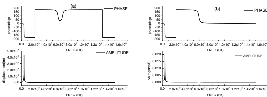
Figure 6. The Displacement and Voltage of the Harvester in Harmonic Analysis
