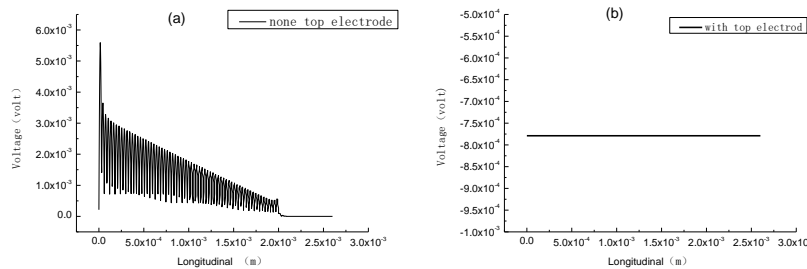
Figure 4. Voltage Generate by the Harvester Under Gravity
