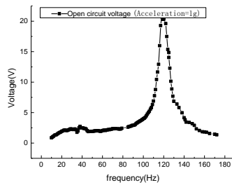
Figure 19. Relationship of Peak Voltage and Frequency
