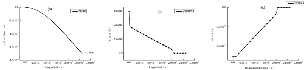
Figure 3. Beam Deflection and the Stress and Strain X Direction
